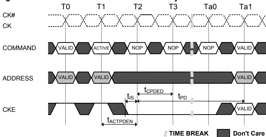
Figure 66. Active Command to Power-Down Entry
