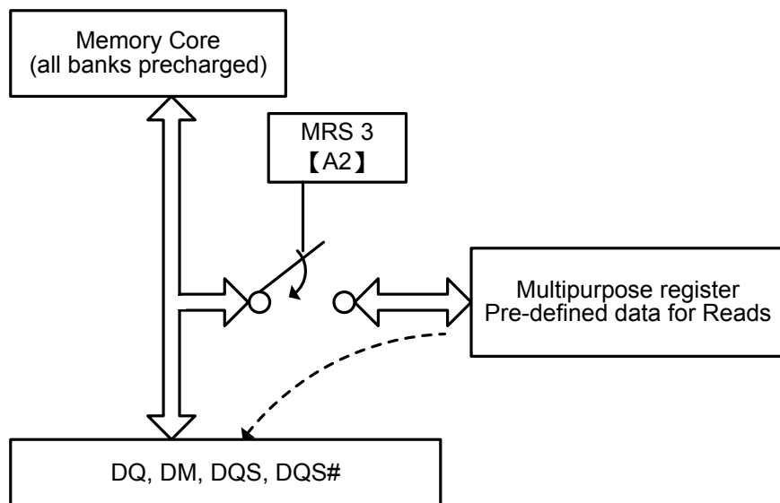
Figure 9. MPR Block Diagram
